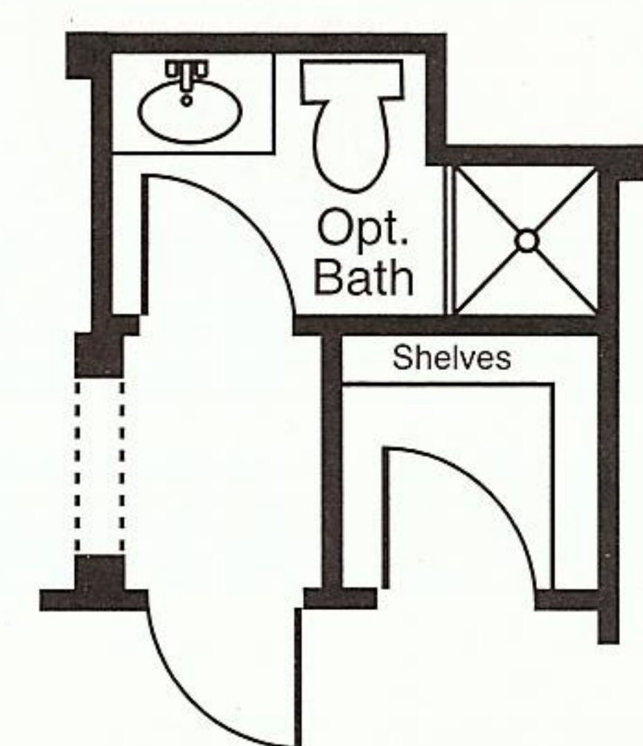
PARTIAL PLAN W/OPT. BATH
