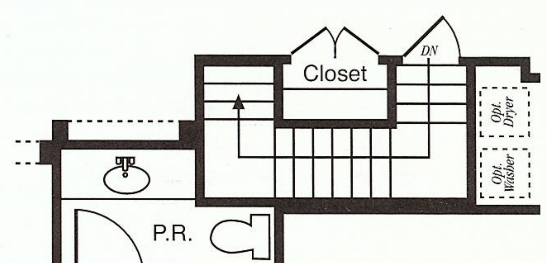
PARTIAL PLAN OPT. BASEMENT CONDITION
